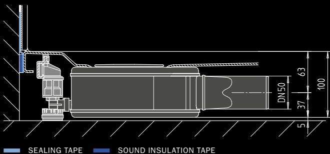
The figure shows: SUPERPLAN ZERO in cross section with foot frame FR 5300 FLEX and waste KA 90 horizontal.
